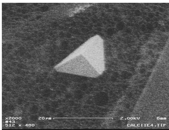
FIG. 5. A scanning electron micrograph of a single tetrahedral crystal oriented base down on a TEM grid. The three basal corners have been cleaved on planes parallel to the upper three faces.
