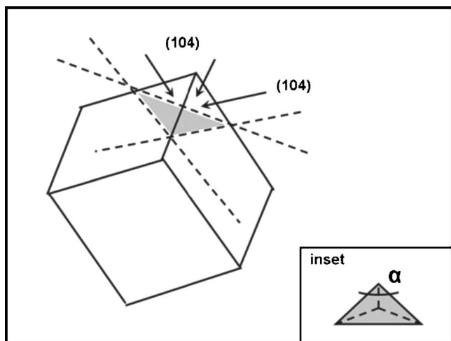
FIG. 6. The intersection of a plane and the corner of a (104) rhombohedral calcite crystal. All arrows indicate (104) crystal planes. The shaded triangle base of the resulting tetrahedron lies on a different plane. The inset shows a view of the tetrahedral crystal from above, with the isosceles angle of the base labeled \alpha .
